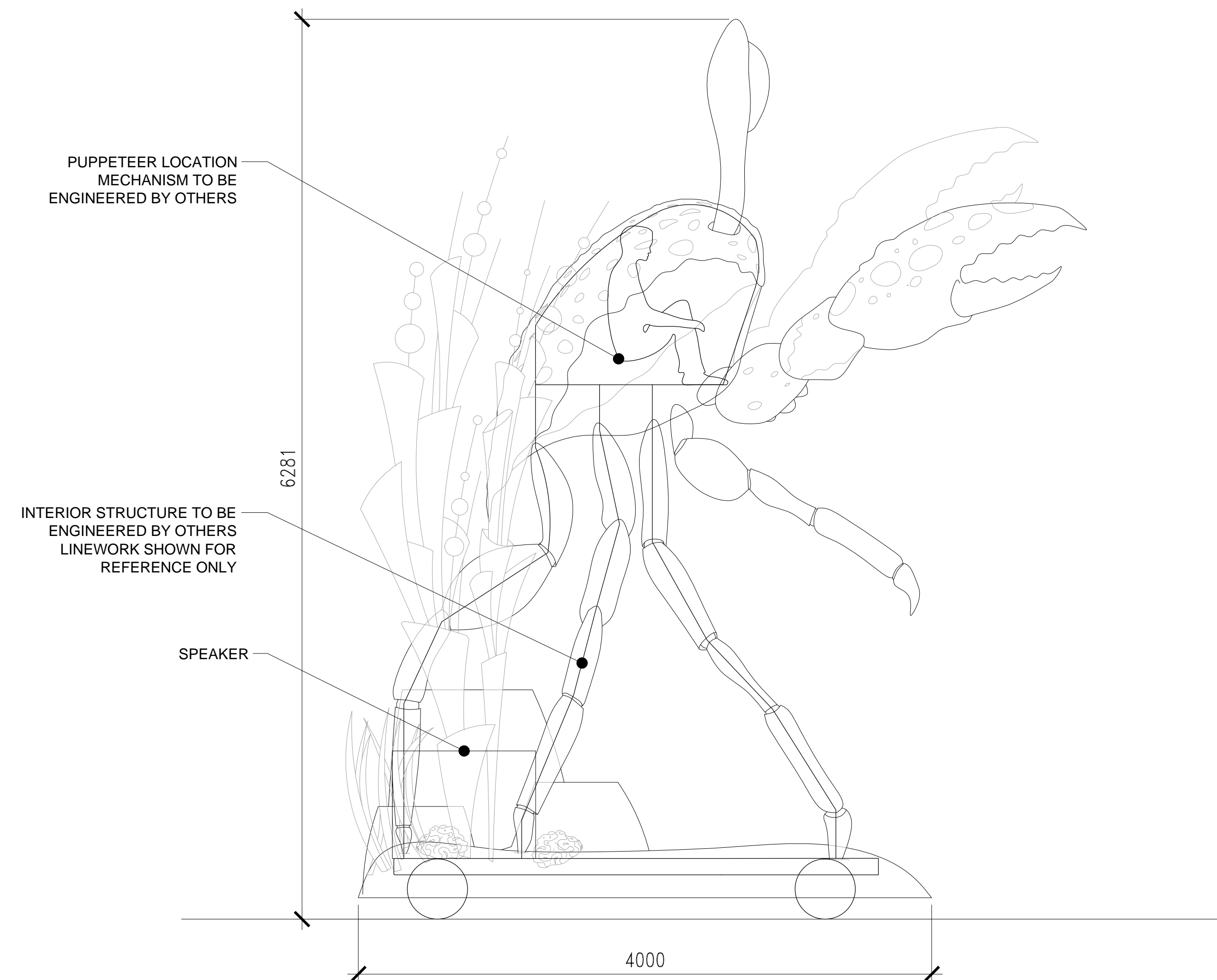
3 CHIMELONG PARADE CRAB CONGA LINE: CRAB PLAN 1:25
