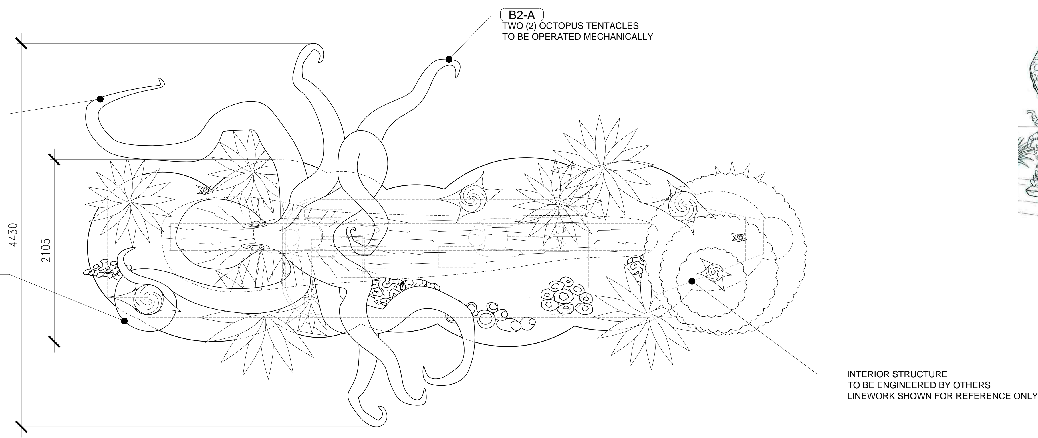
5 CHIMELONG PARADE CORAL REEF: OCTOPUS PLAN 1:25
