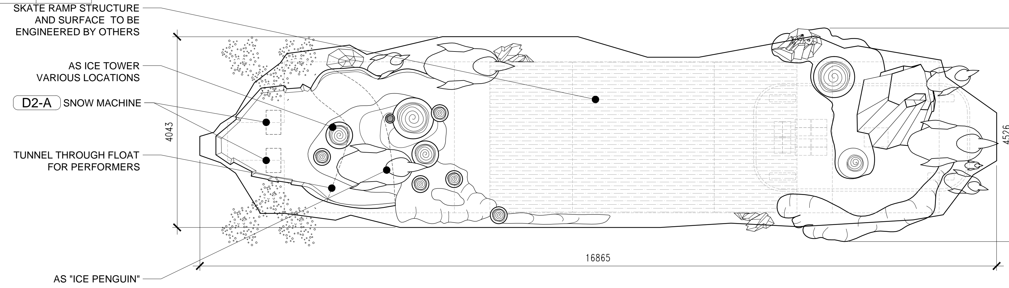
2 CHIMELONG PARADE POLAR GAMES PLAN 1:50
