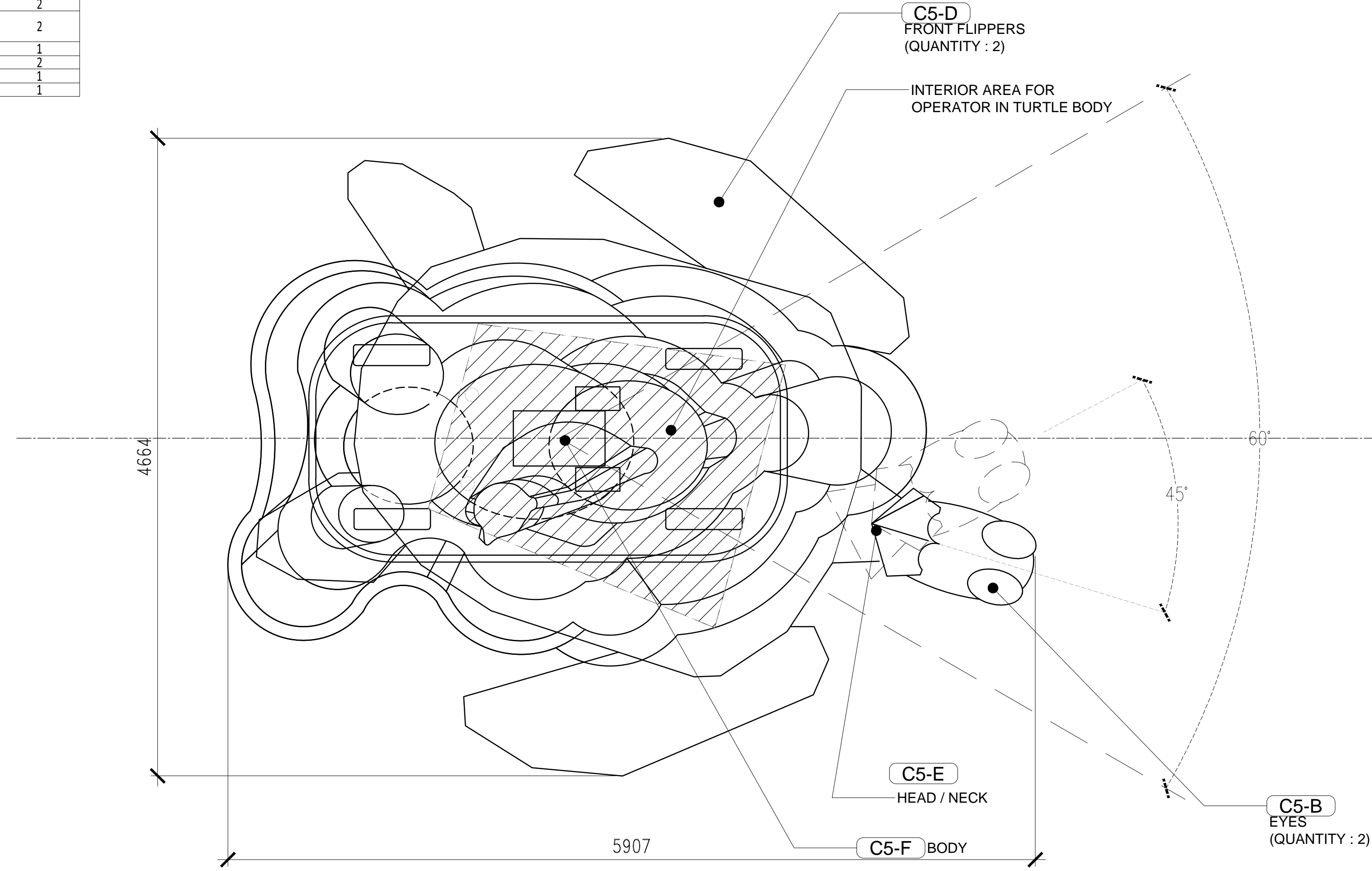
2 CHIMELONG PARADE LARGE TURTLE PLAN 1:25
