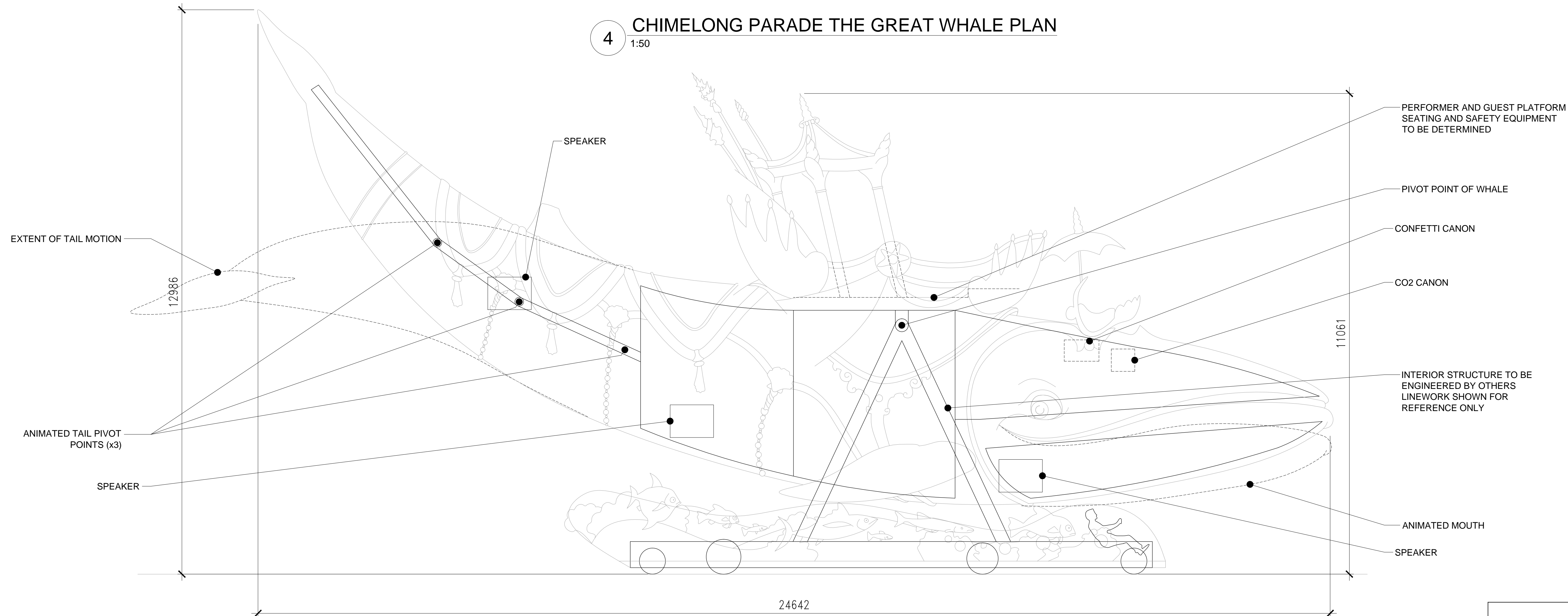
3 CHIMELONG PARADE THE GREAT WHALE ELEVATION 1:50
