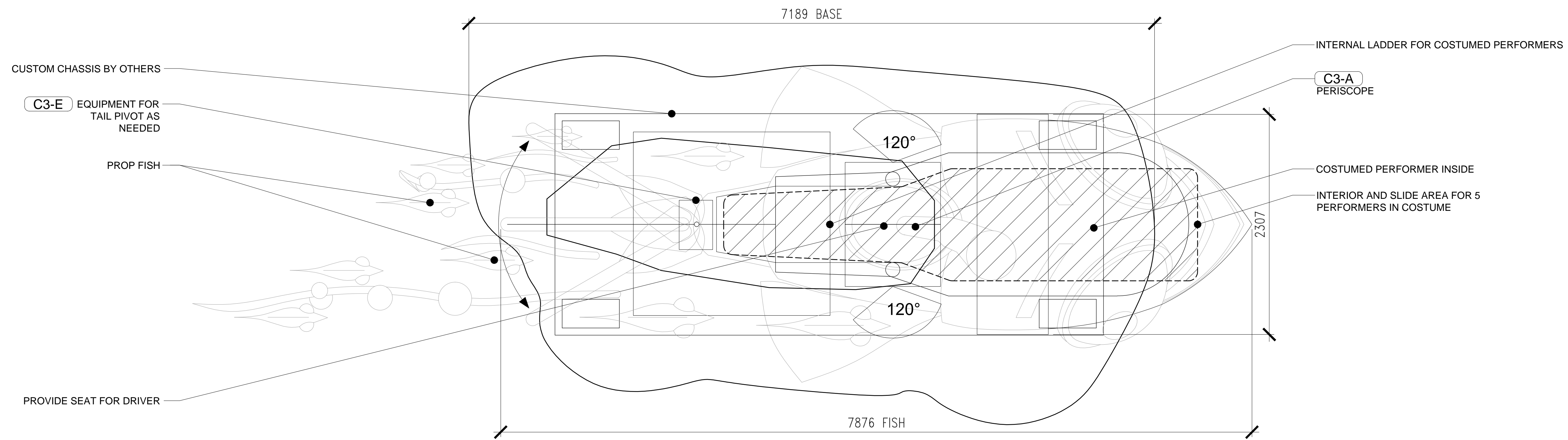
3 CHIMELONG PARADE SUBMARINE PLAN 1:25
