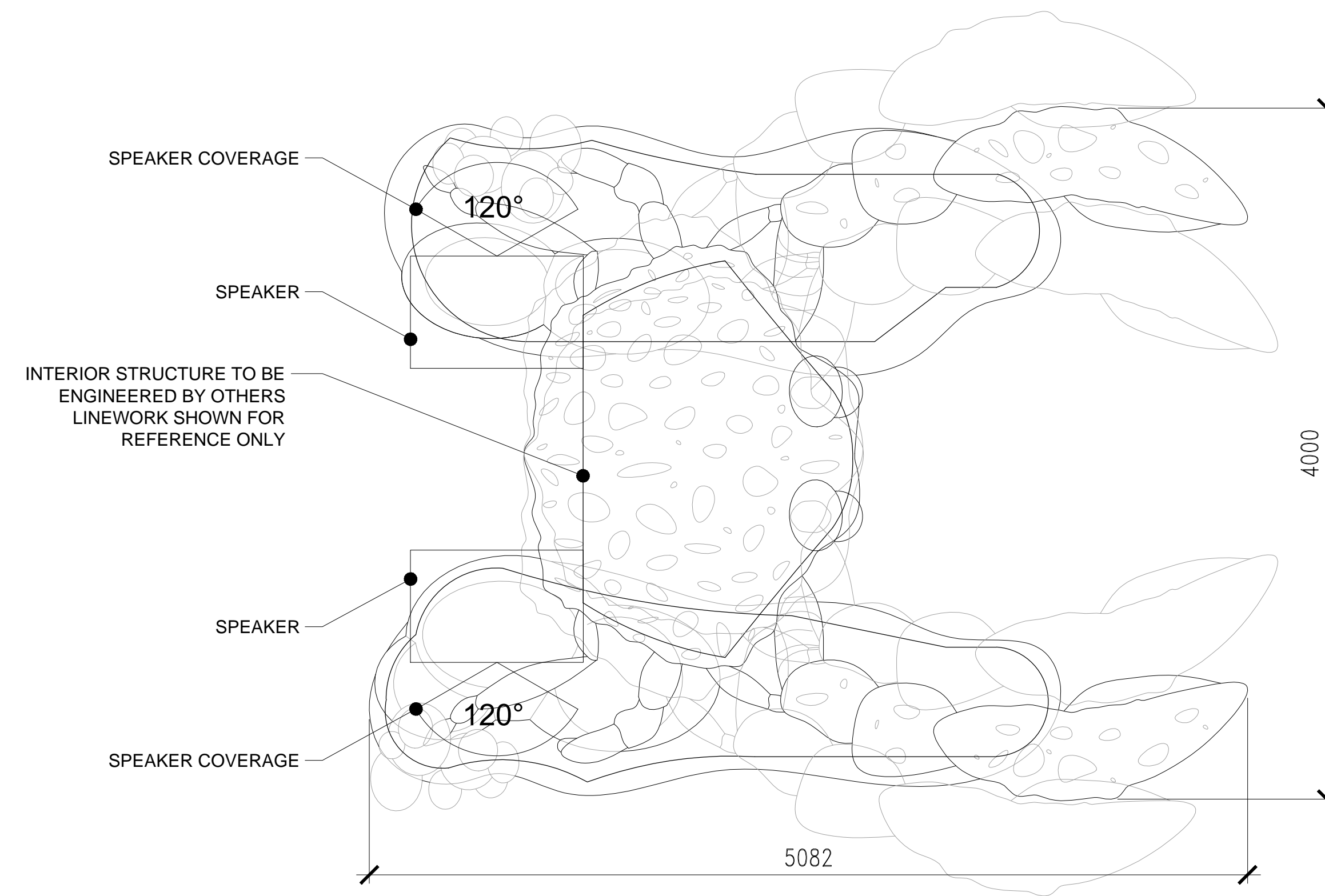
4 CHIMELONG PARADE CRAB CONGA LINE: CRAB PLAN 1:25
