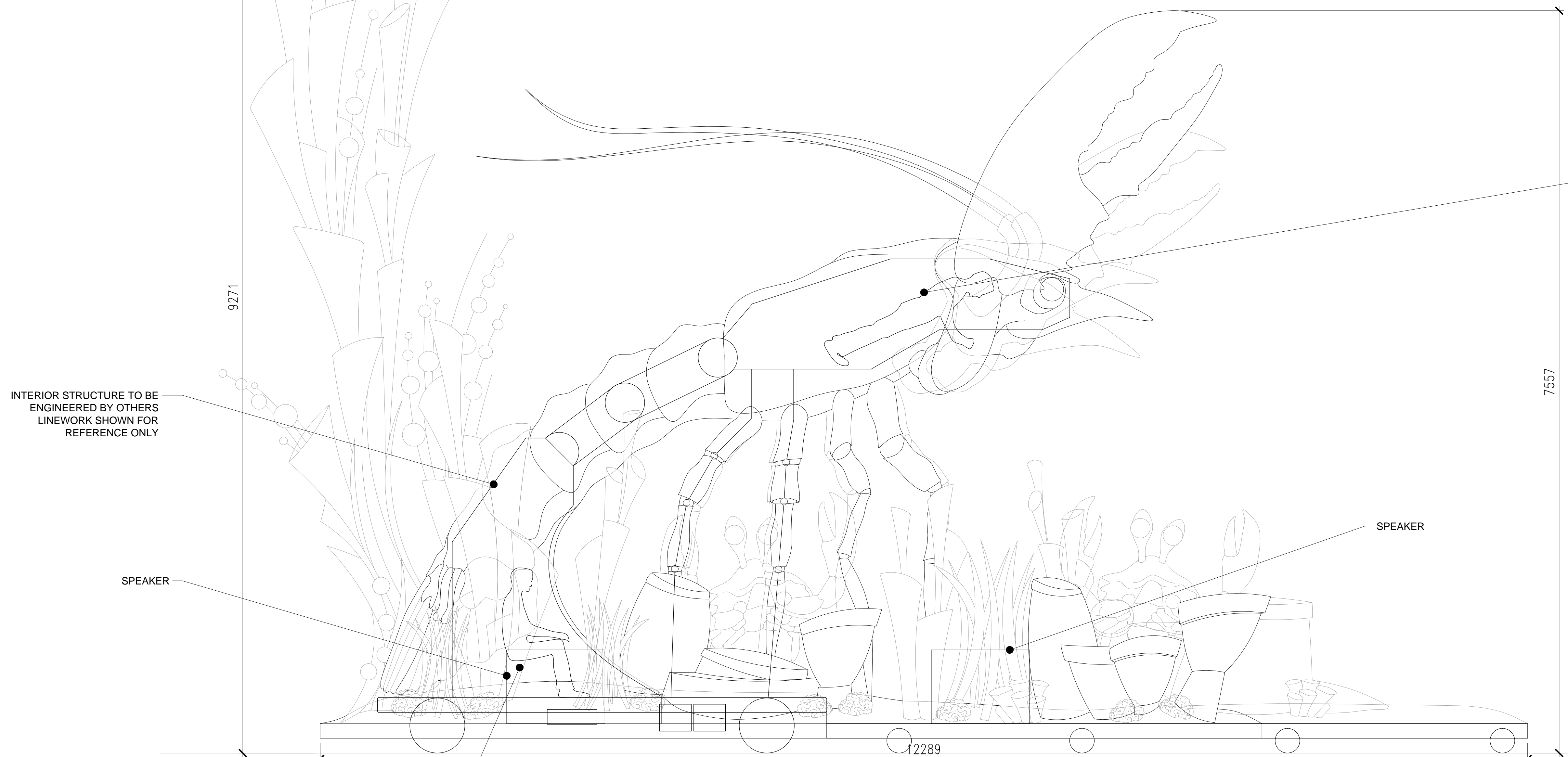
3 CHIMELONG PARADE CRUSTACEAN CARNIVAL PLAN 1:50
