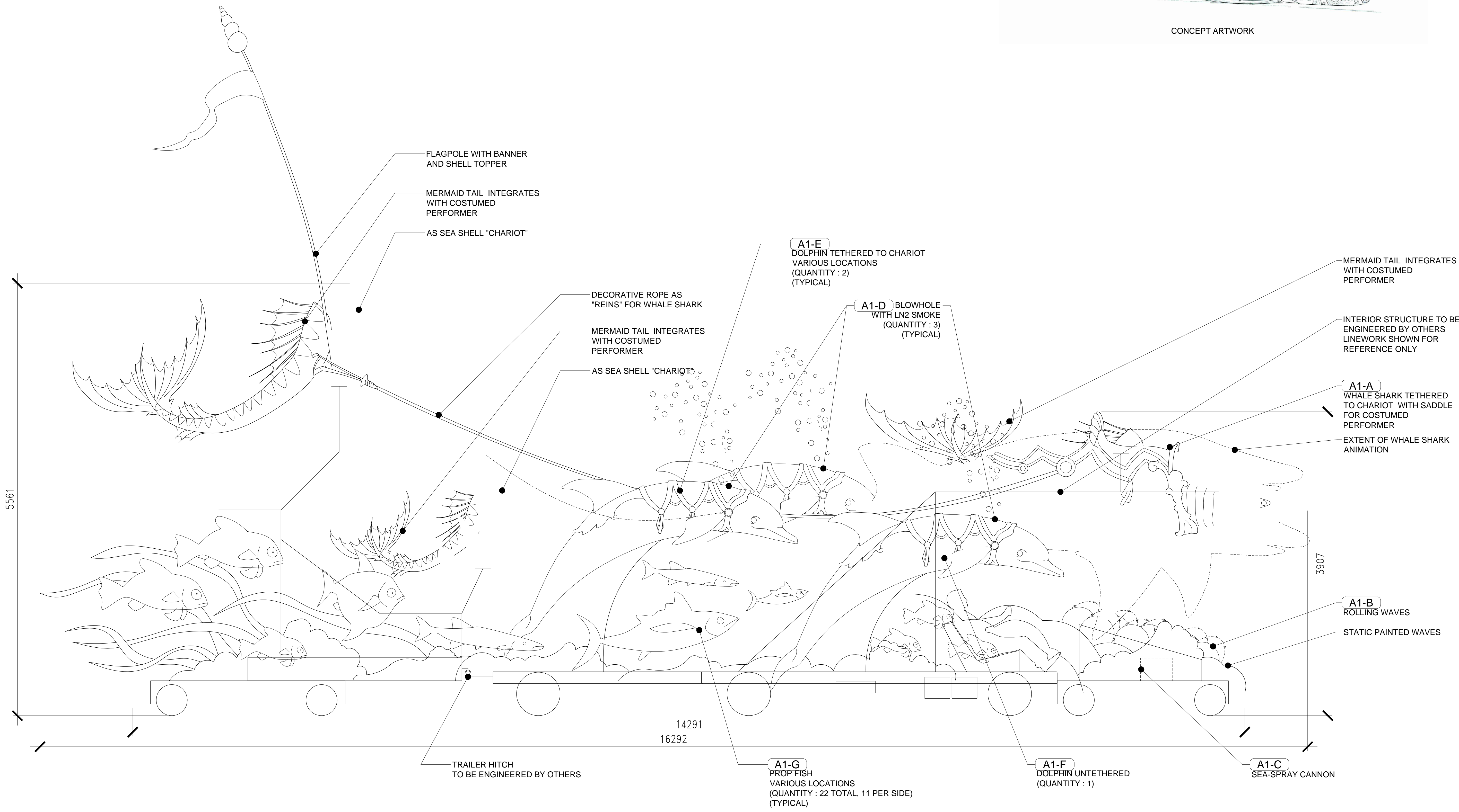
1 CHIMELONG PARADE FANFARE ELEVATION 1:25
