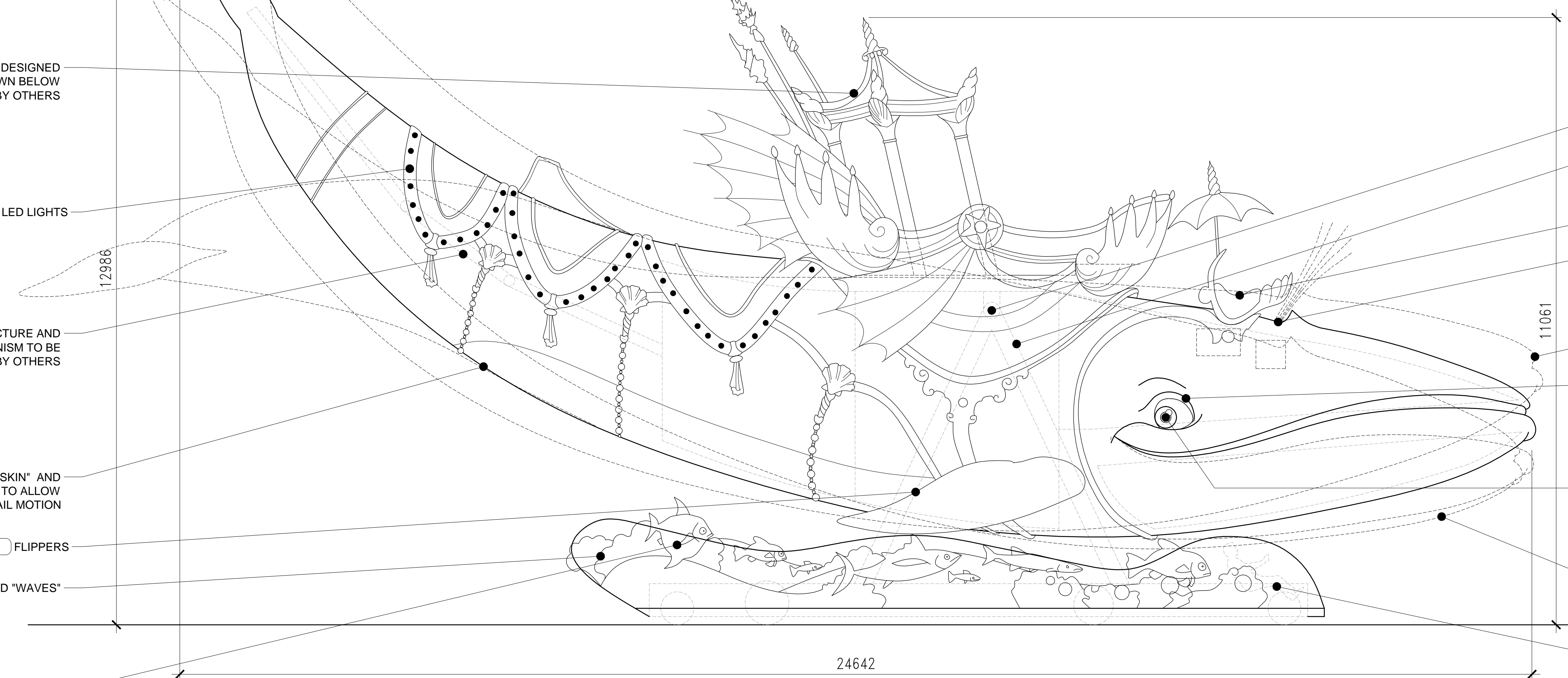
2 CHIMELONG PARADE THE GREAT WHALE ELEVATION 1:50
