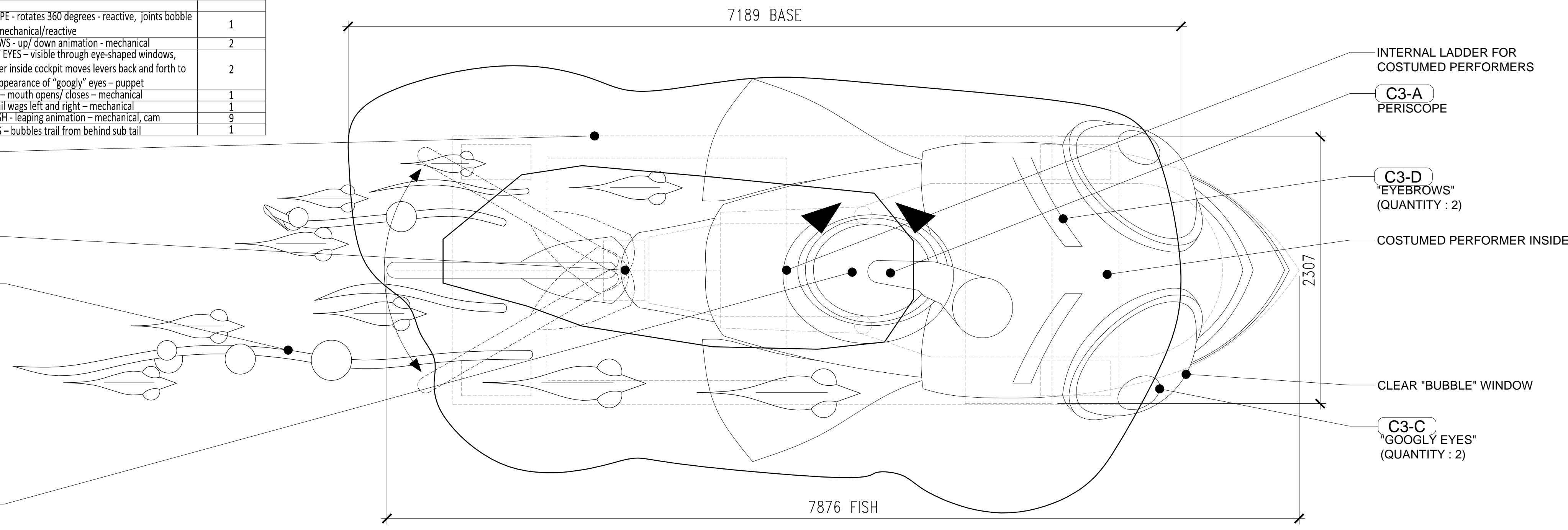
2 CHIMELONG PARADE SUBMARINE PLAN 1:25
