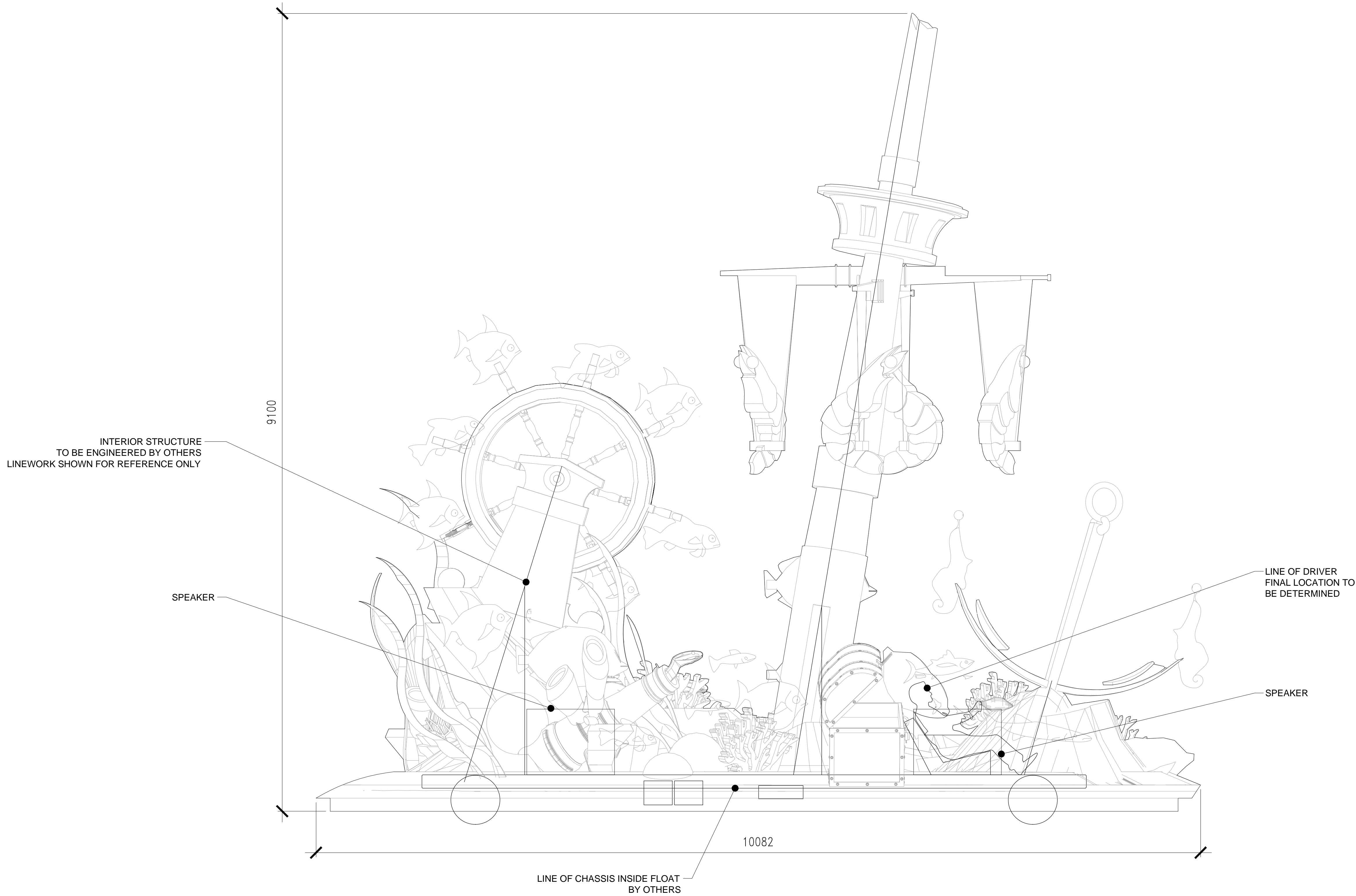
2 CHIMELONG PARADE SHIPWRECK PLAYGROUND ELEVATION 1:25
