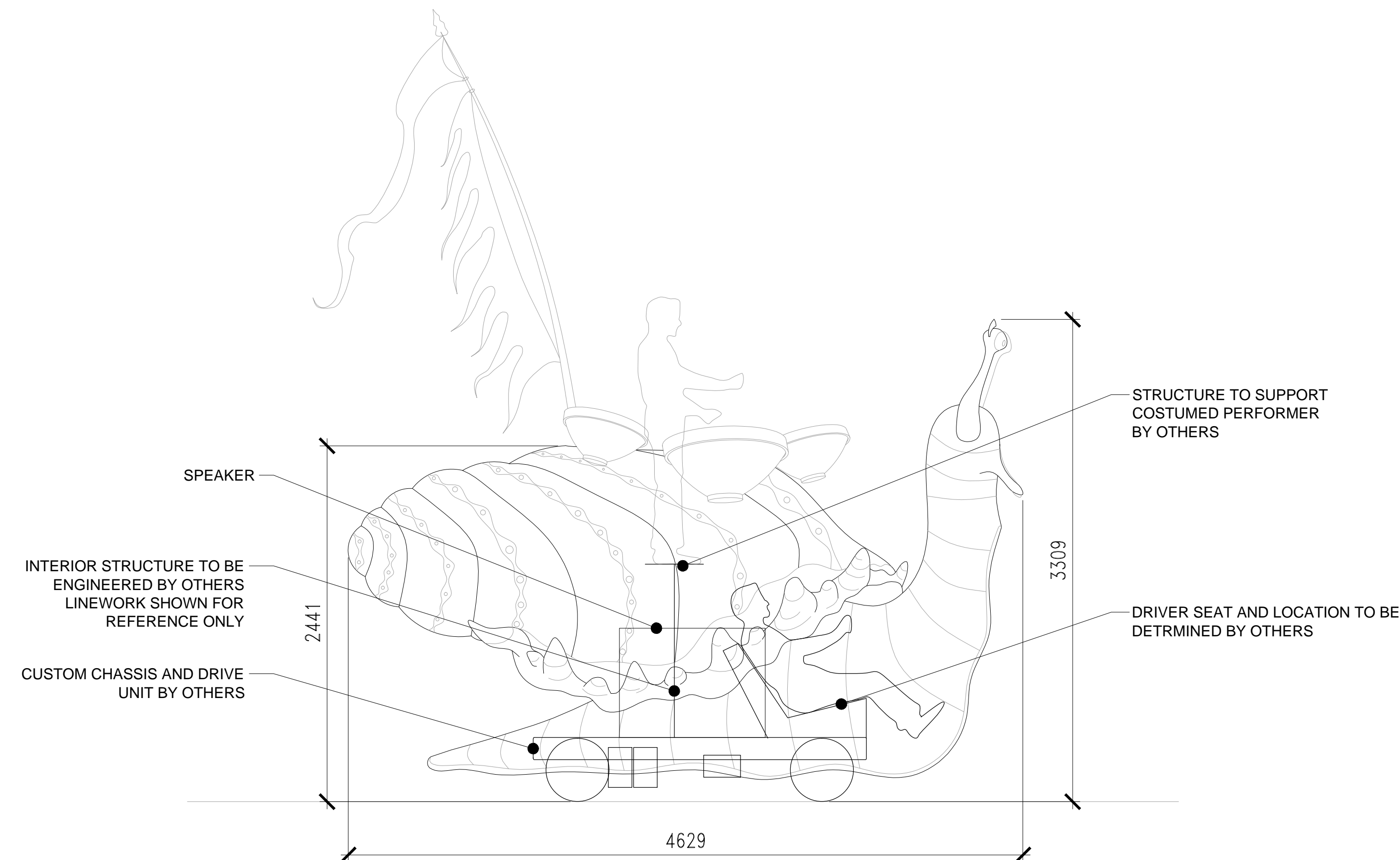
3 CHIMELONG PARADE CRAB CONGA LINE: SEA SNAIL ELEVATION 1:25
