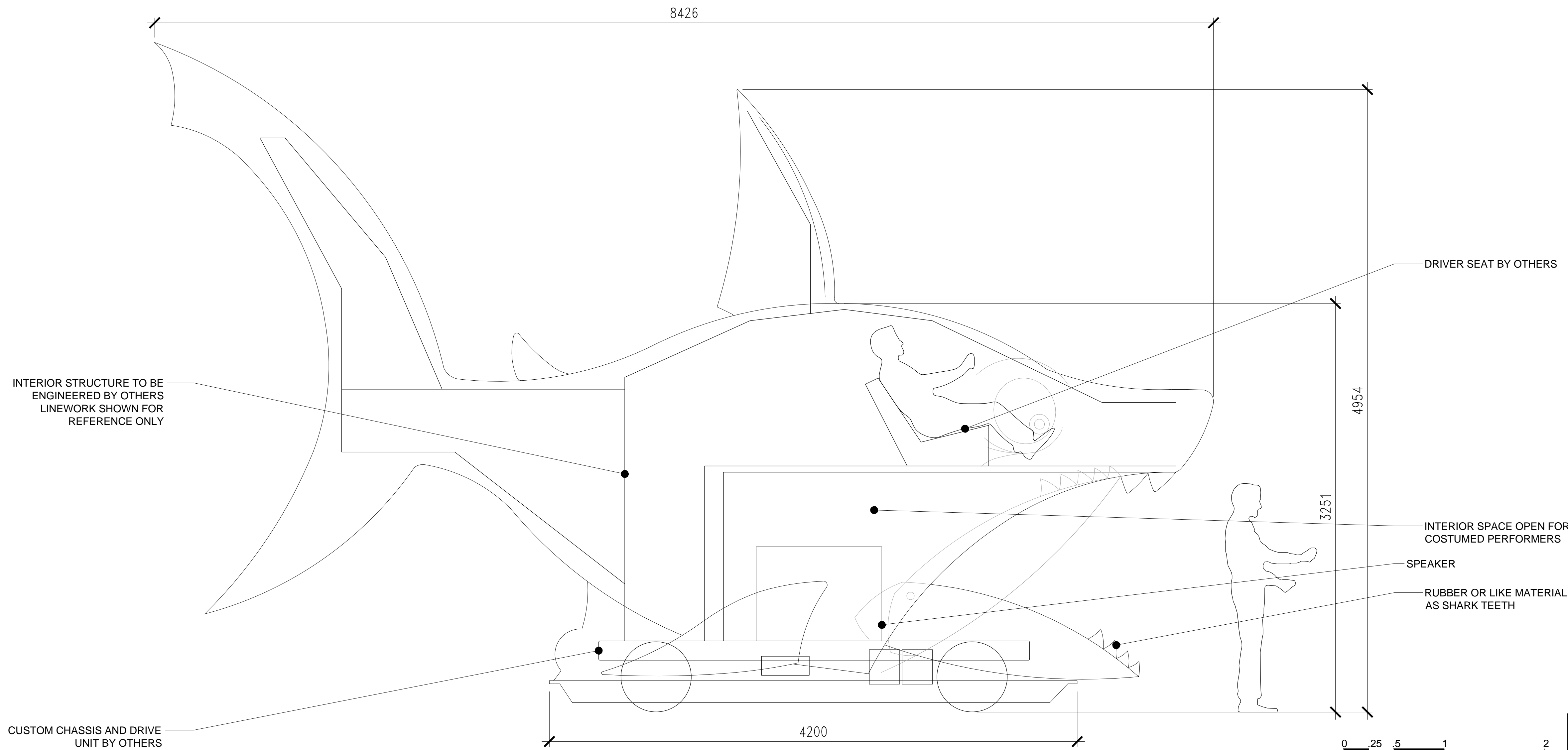
3 CHIMELONG PARADE SILLY SHARK ELEVATION 1:25
