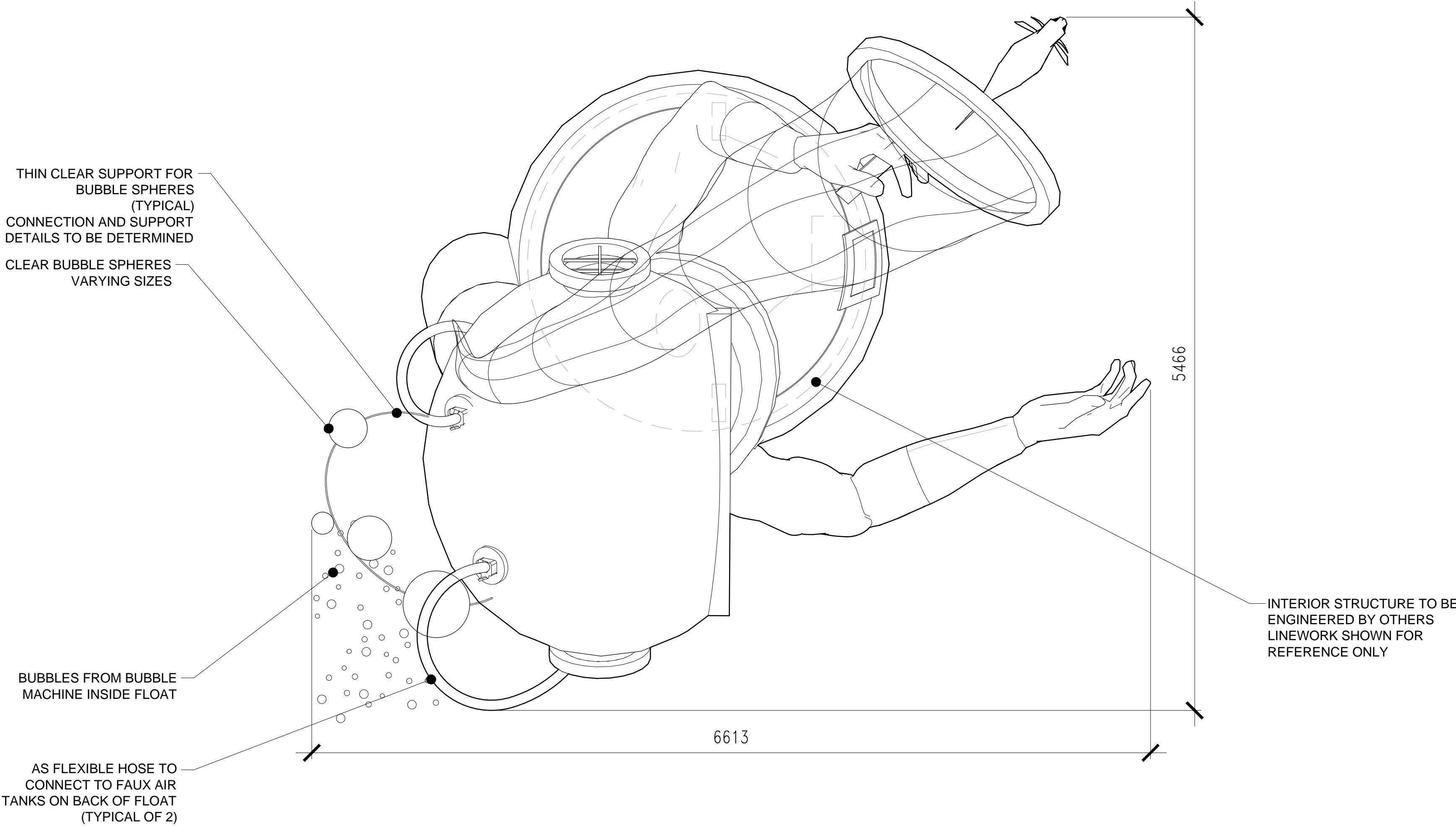
2 CHIMELONG PARADE DIVER PLAN 1:25
