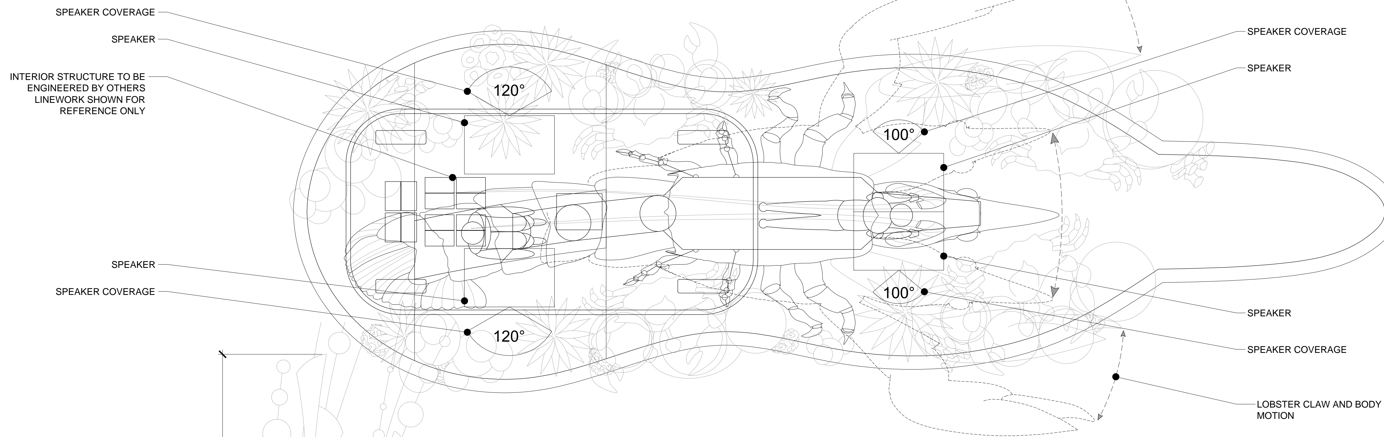
4 CHIMELONG PARADE CRUSTACEAN CARNIVAL PLAN 1:50
