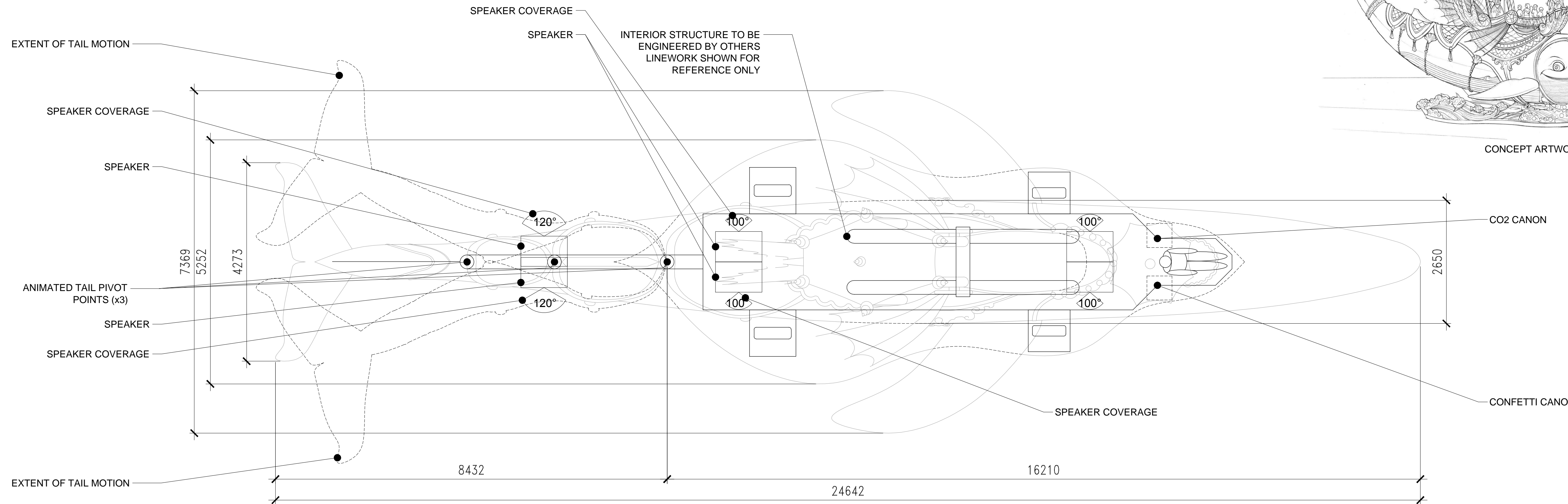
4 CHIMELONG PARADE THE GREAT WHALE PLAN 1:50
