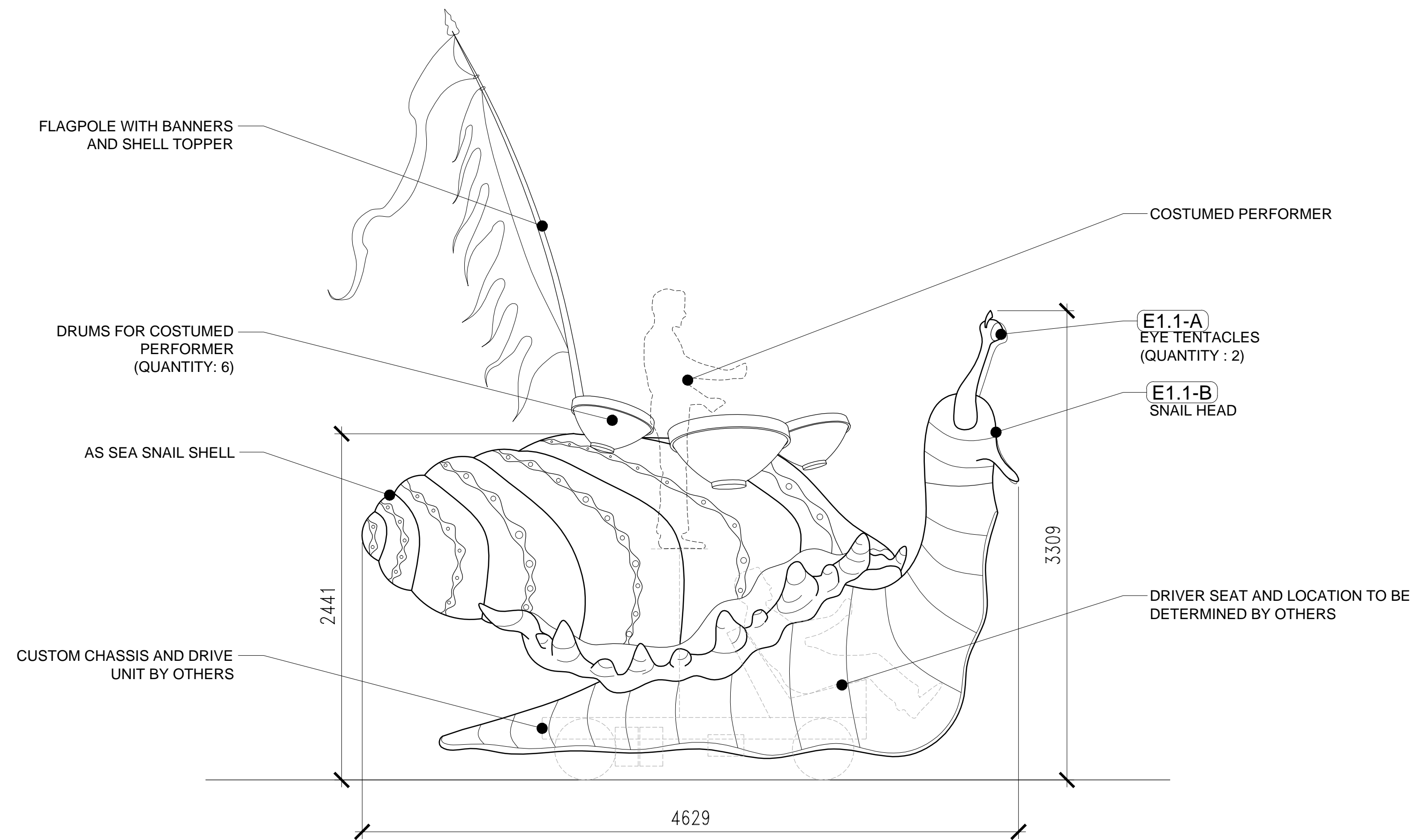
1 CHIMELONG PARADE CRAB CONGA LINE: SEA SNAIL ELEVATION 1:25
