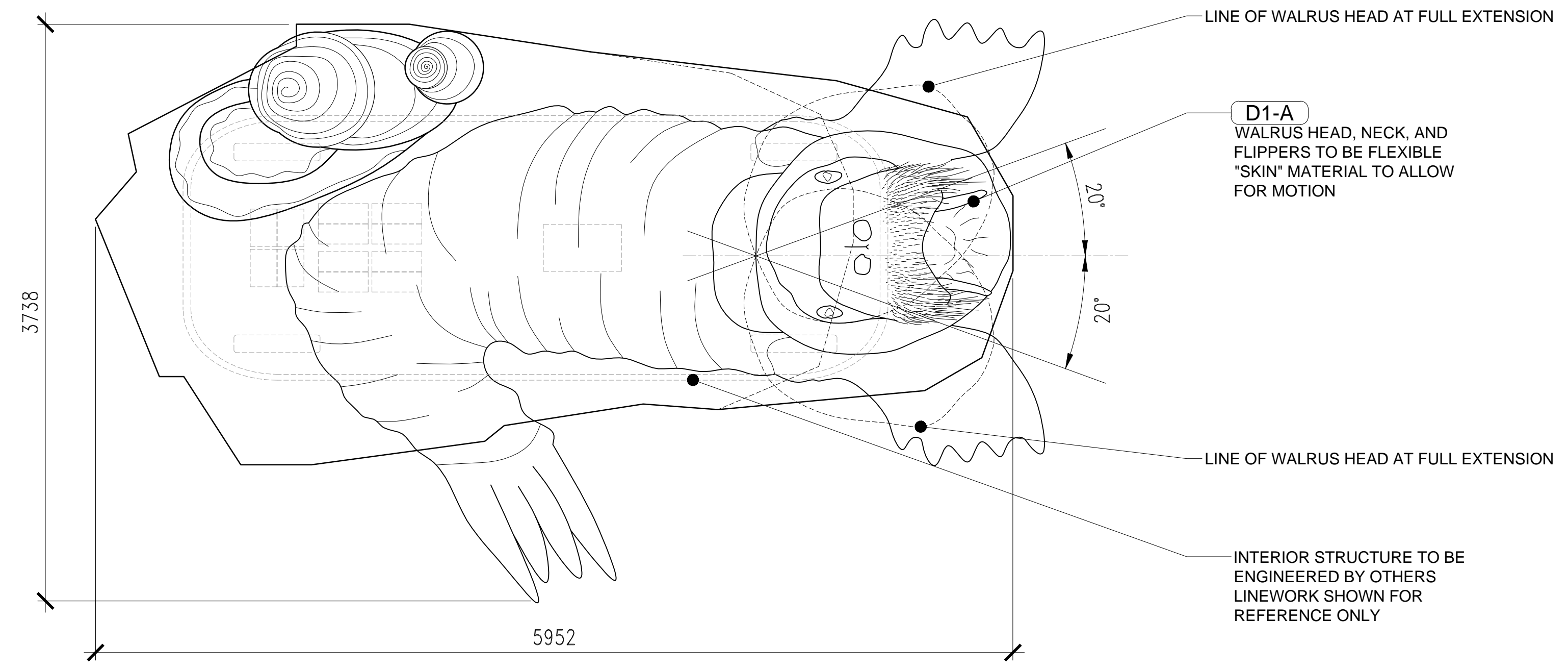
2 CHIMELONG PARADE WALRUS PLAN 1:25
