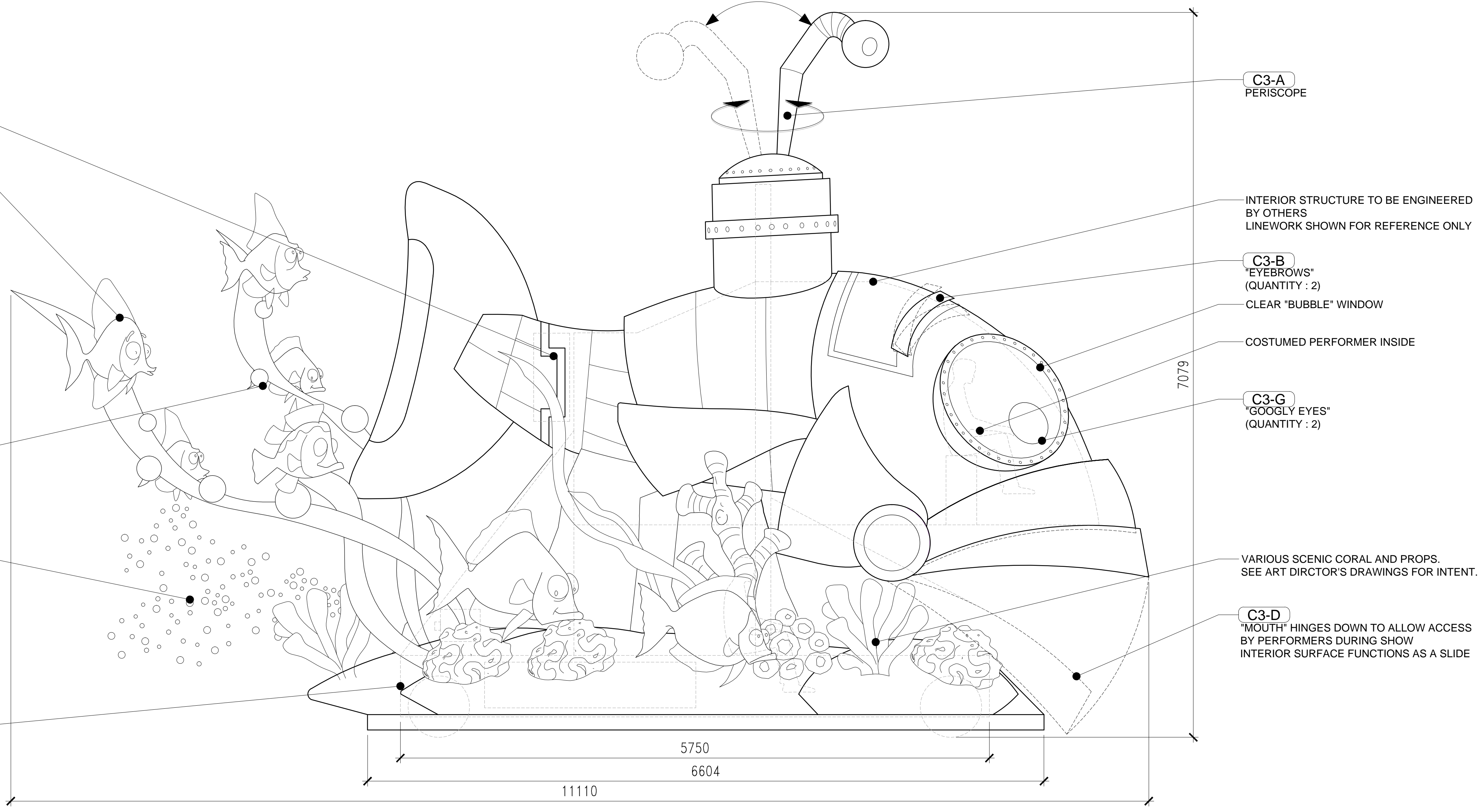
1 CHIMELONG PARADE SUBMARINE ELEVATION 1:25
