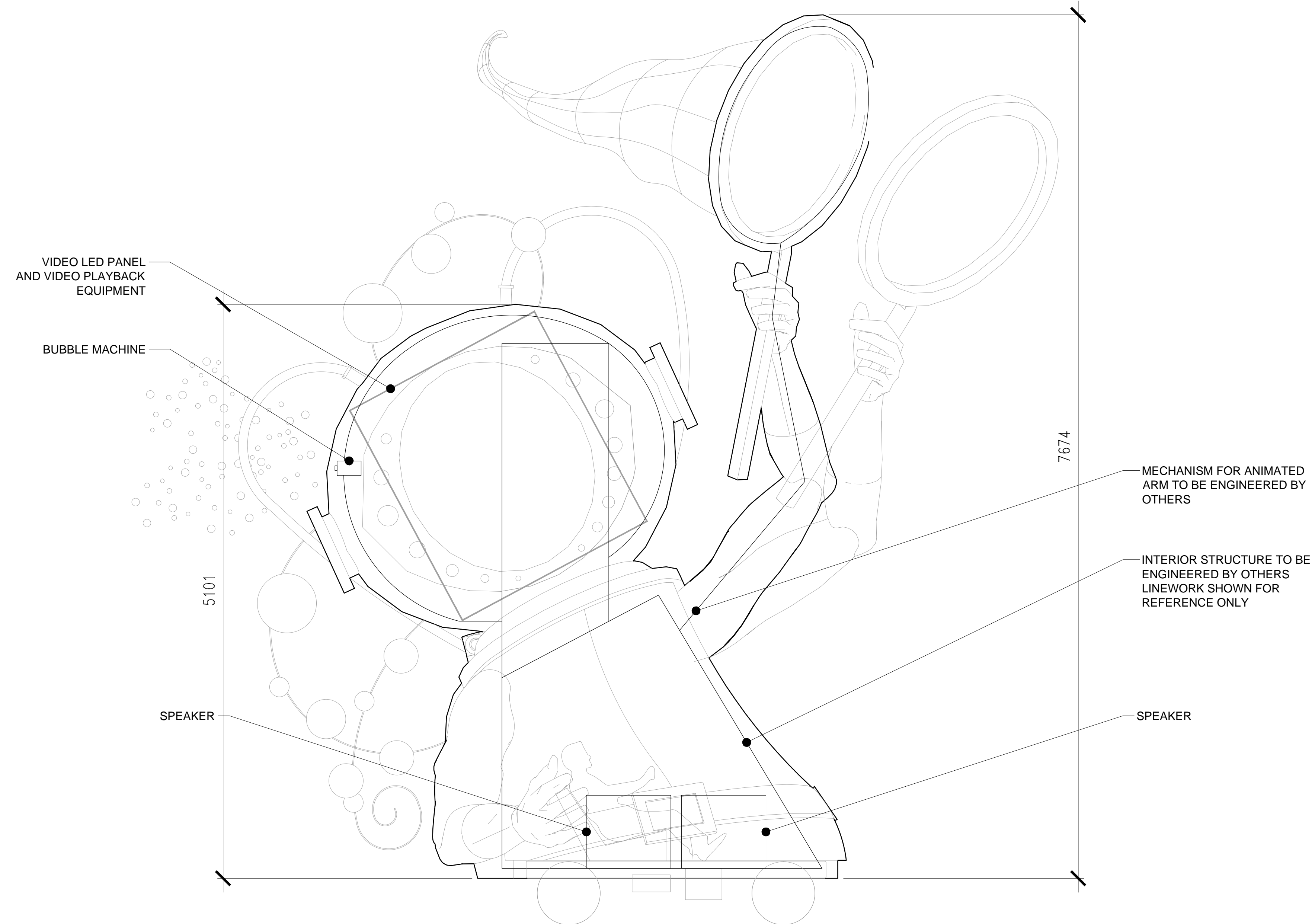
3 CHIMELONG PARADE DIVER ELEVATION 1:25
