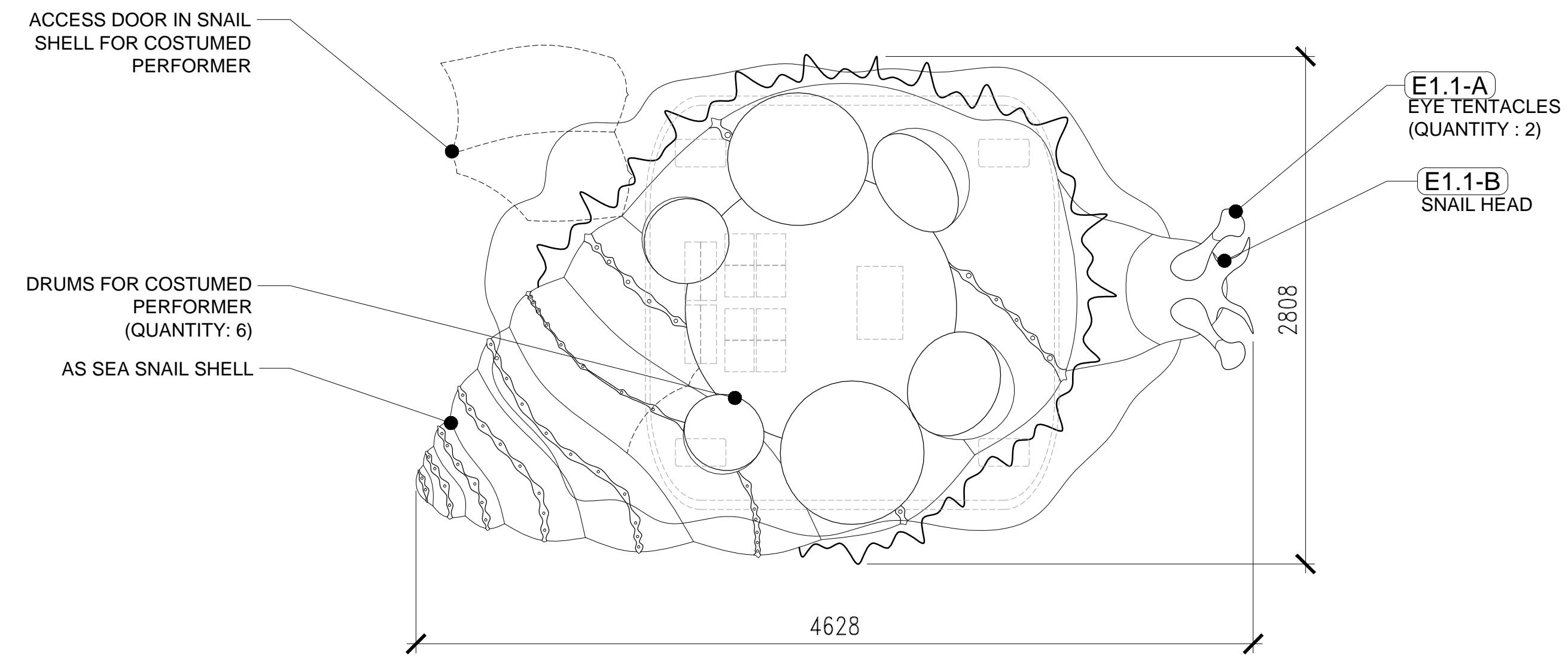
2 CHIMELONG PARADE CRAB CONGA LINE: SEA SNAIL PLAN 1:25
