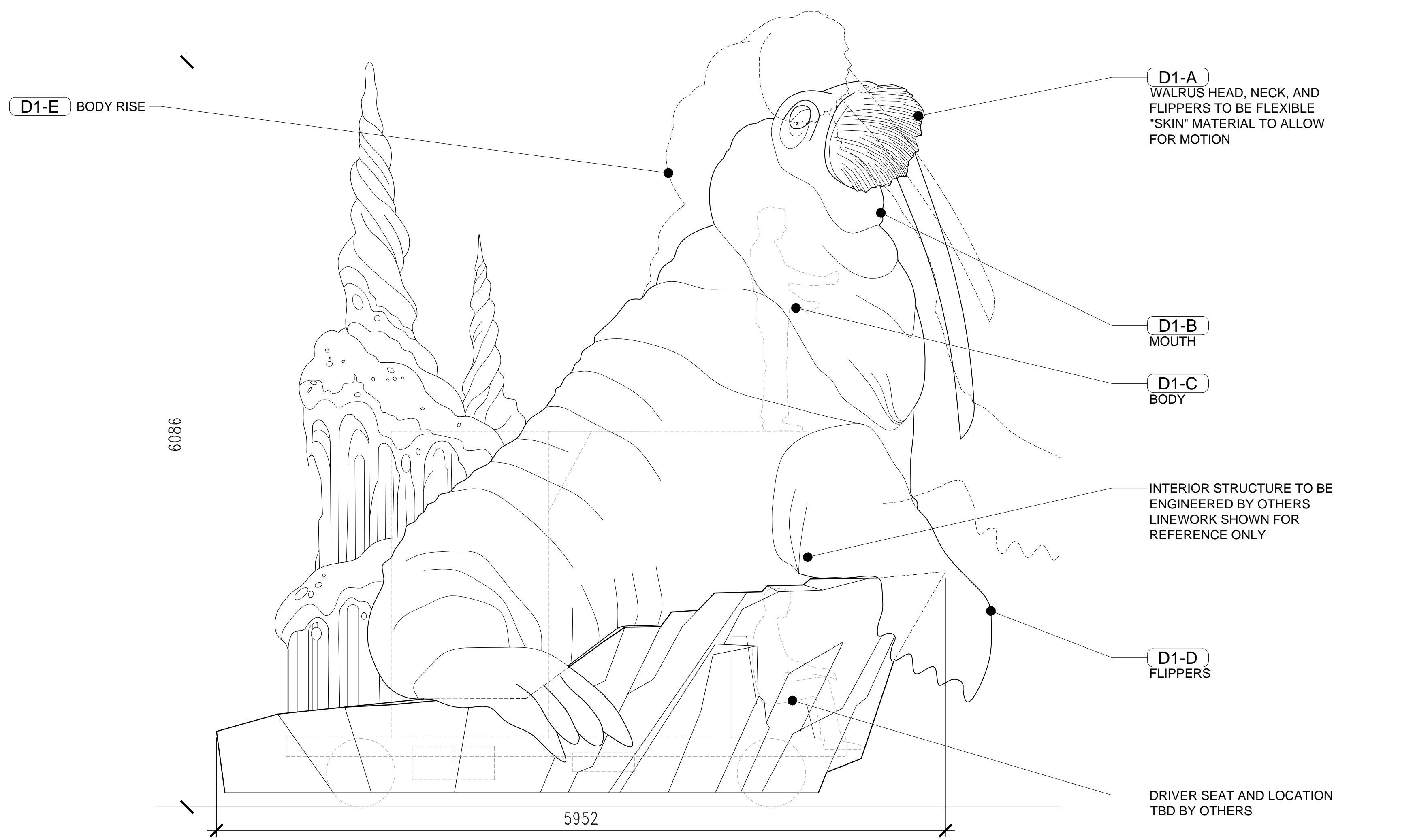
1 CHIMELONG PARADE WALRUS ELEVATION 1:25
