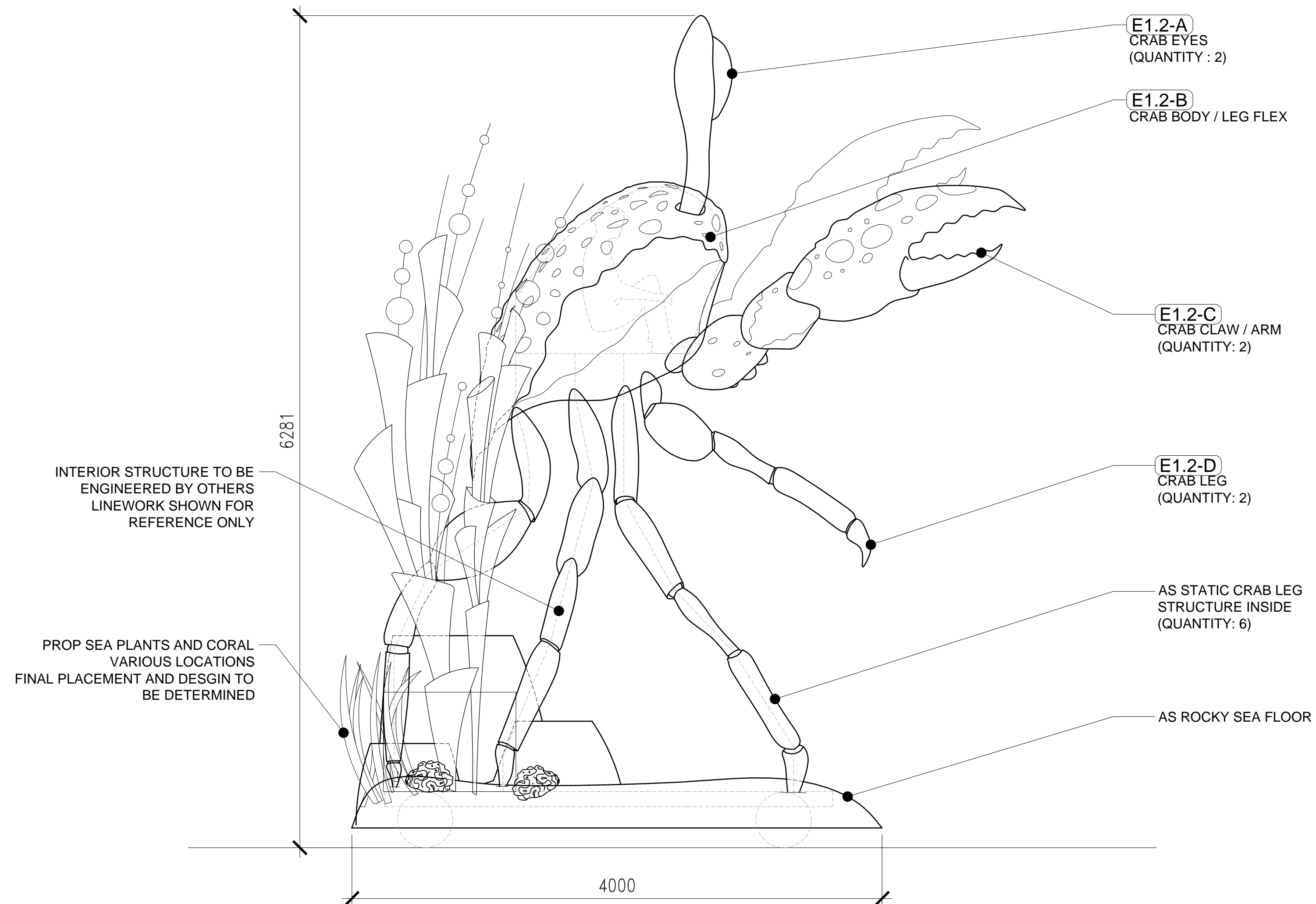
1 CHIMELONG PARADE CRAB CONGA LINE: CRAB PLAN 1:25
