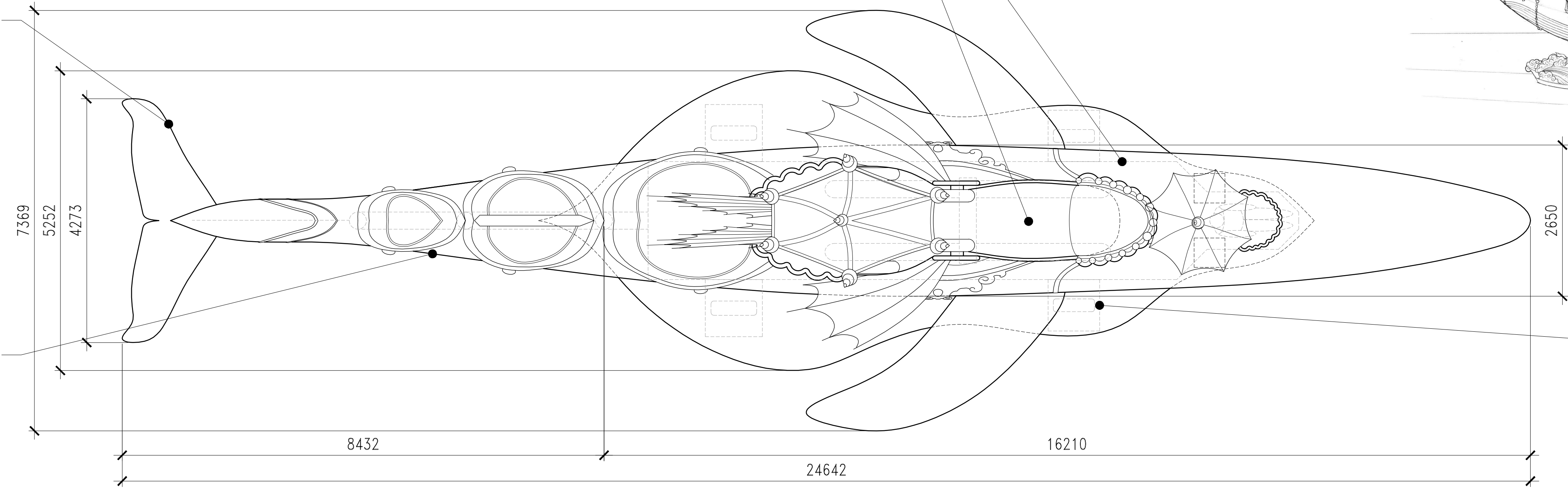
1 CHIMELONG PARADE THE GREAT WHALE PLAN 1:50
