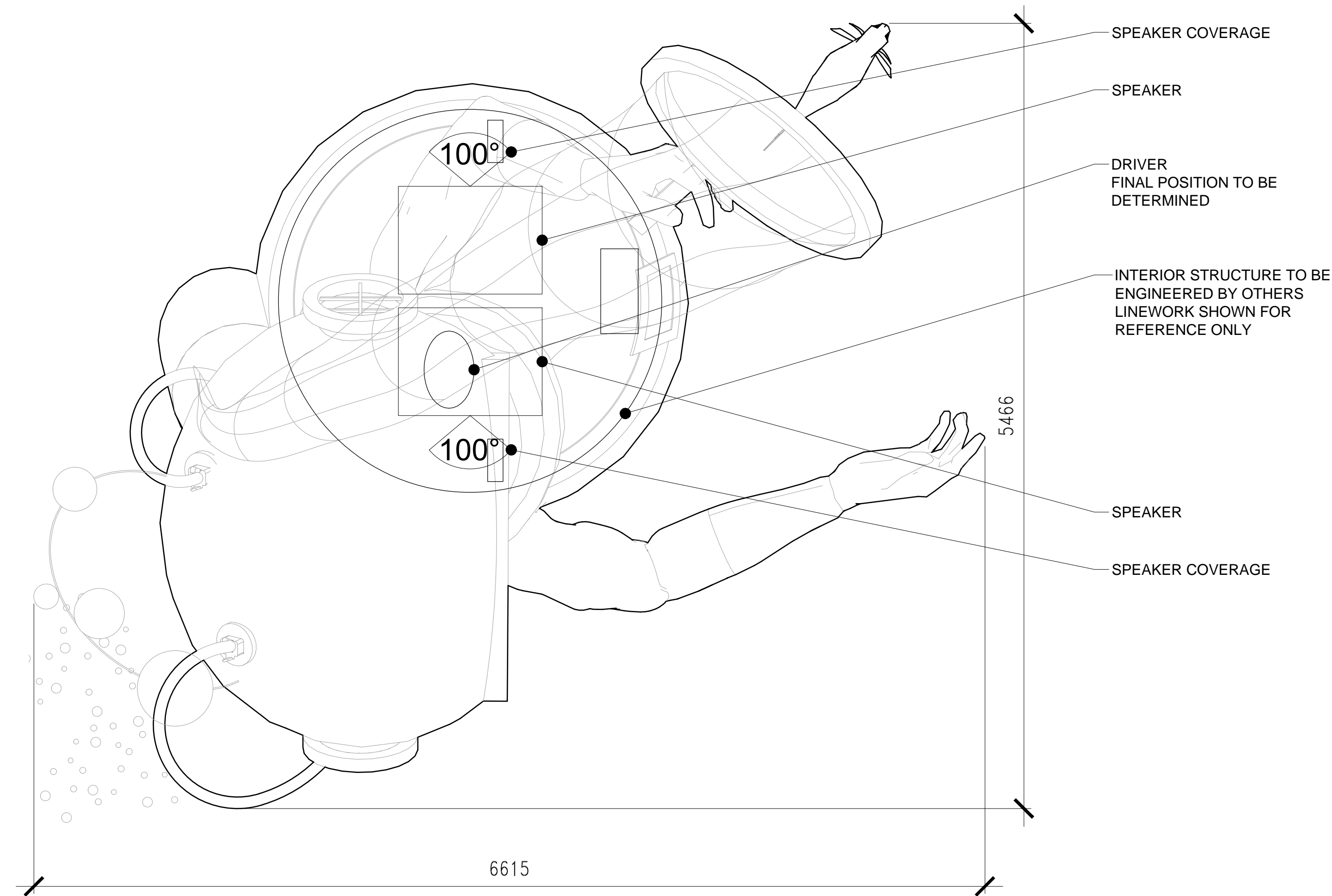
4 CHIMELONG PARADE DIVER PLAN 1:25
