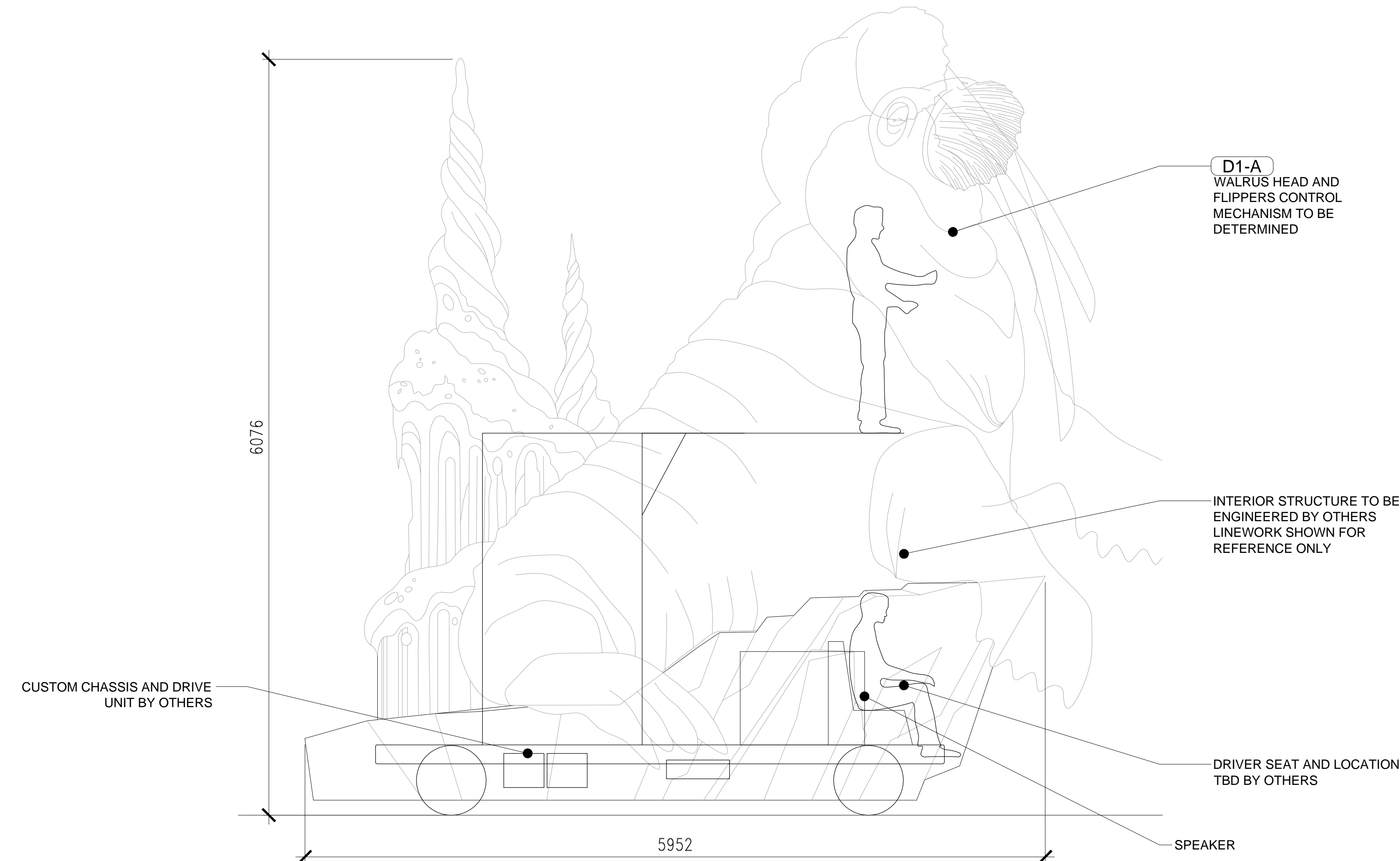
3 CHIMELONG PARADE WALRUS ELEVATION 1:25
