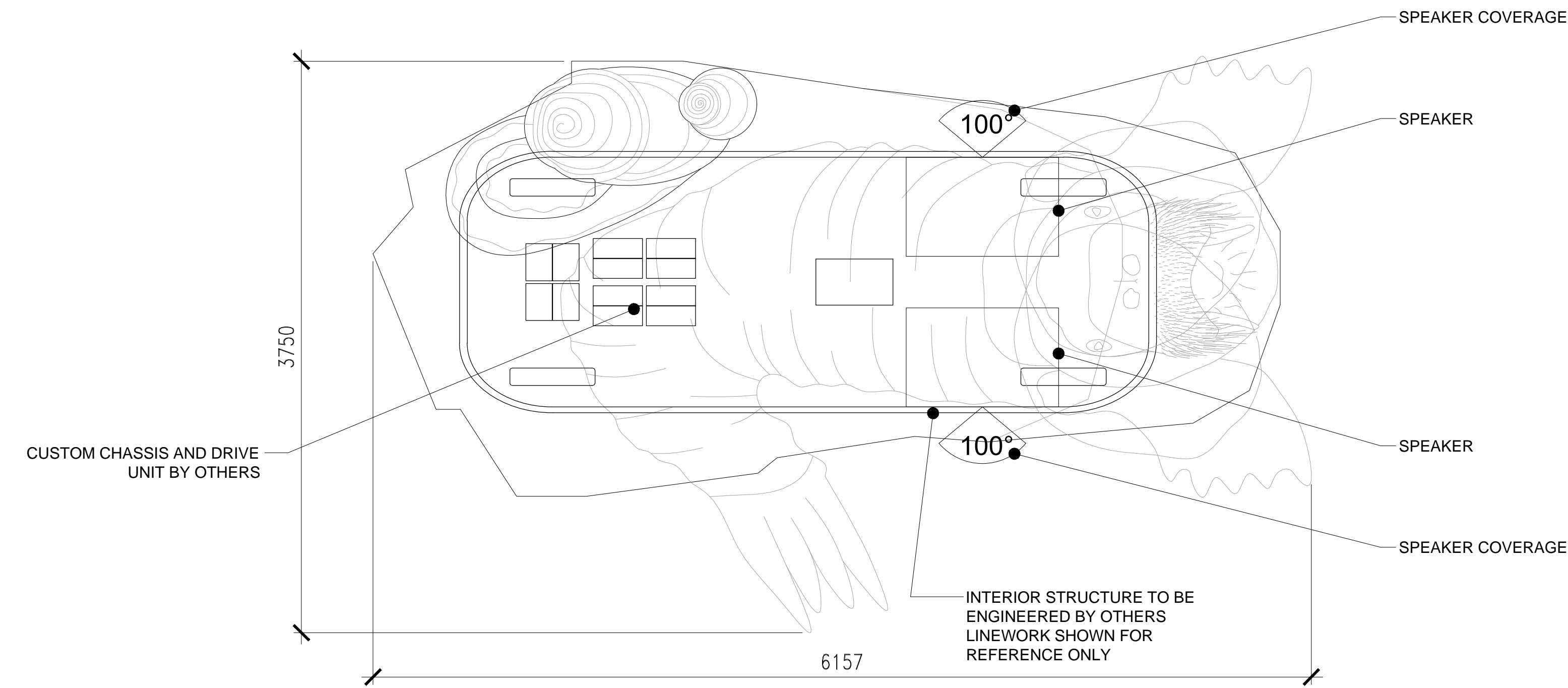
4 CHIMELONG PARADE WALRUS PLAN 1:25
