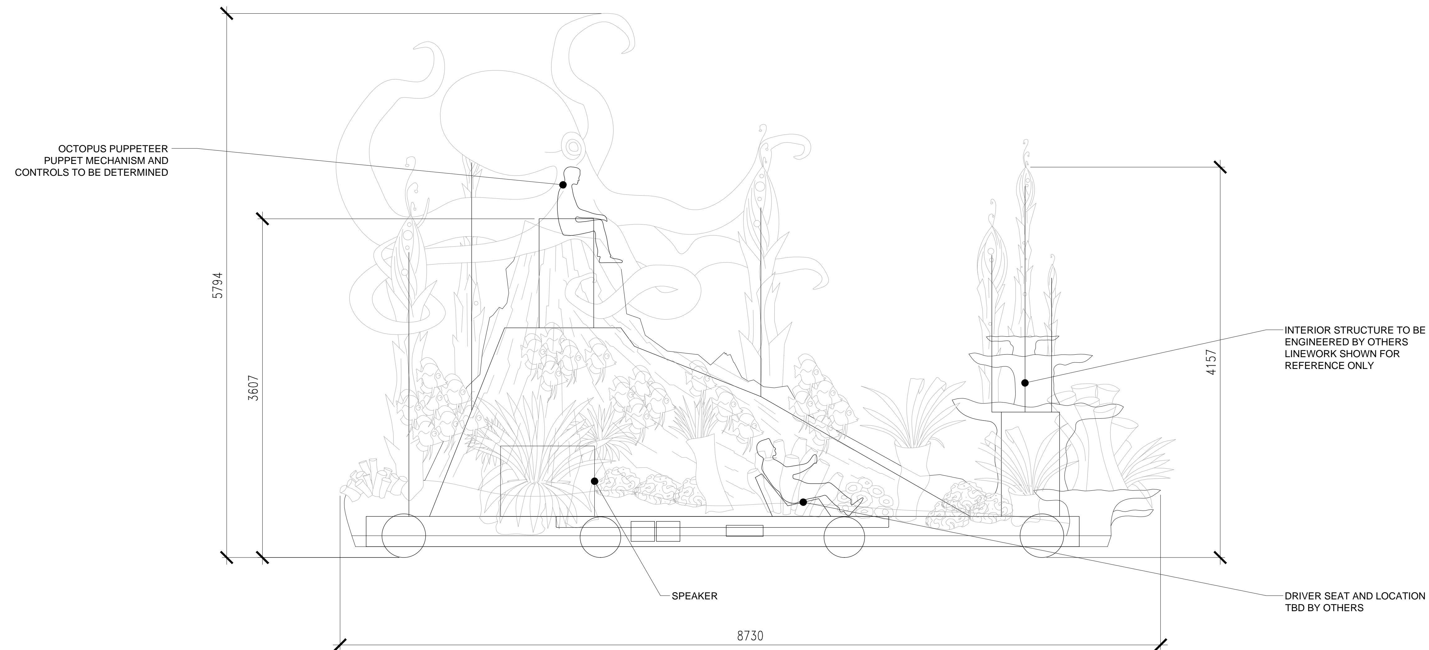
8 CHIMELONG PARADE CORAL REEF: OCTOPUS ELEVATION 1:25
