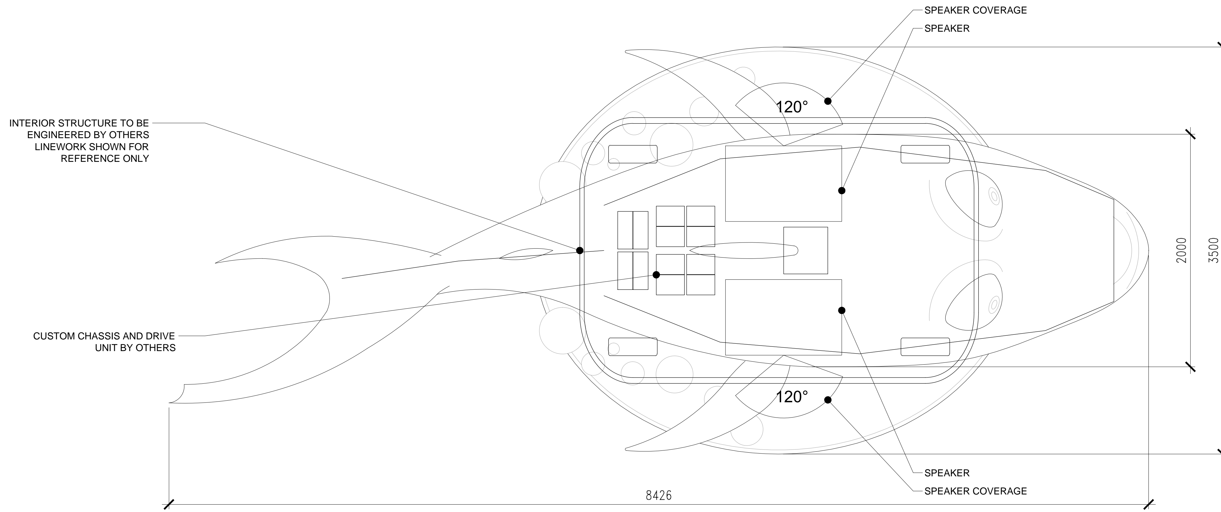
4 CHIMELONG PARADE SILLY SHARK PLAN 1:25
