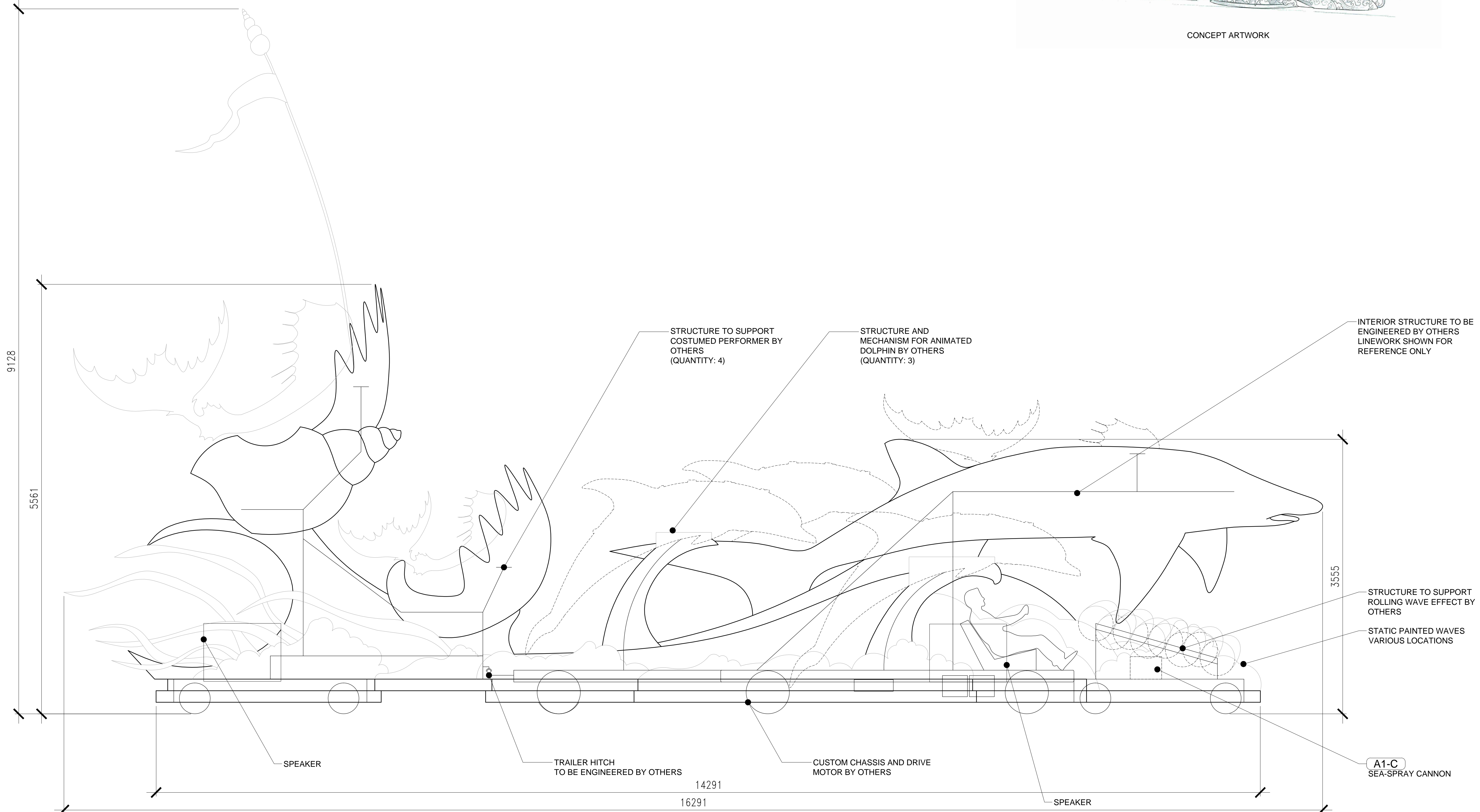
2 CHIMELONG PARADE FANFARE ELEVATION 1:25
