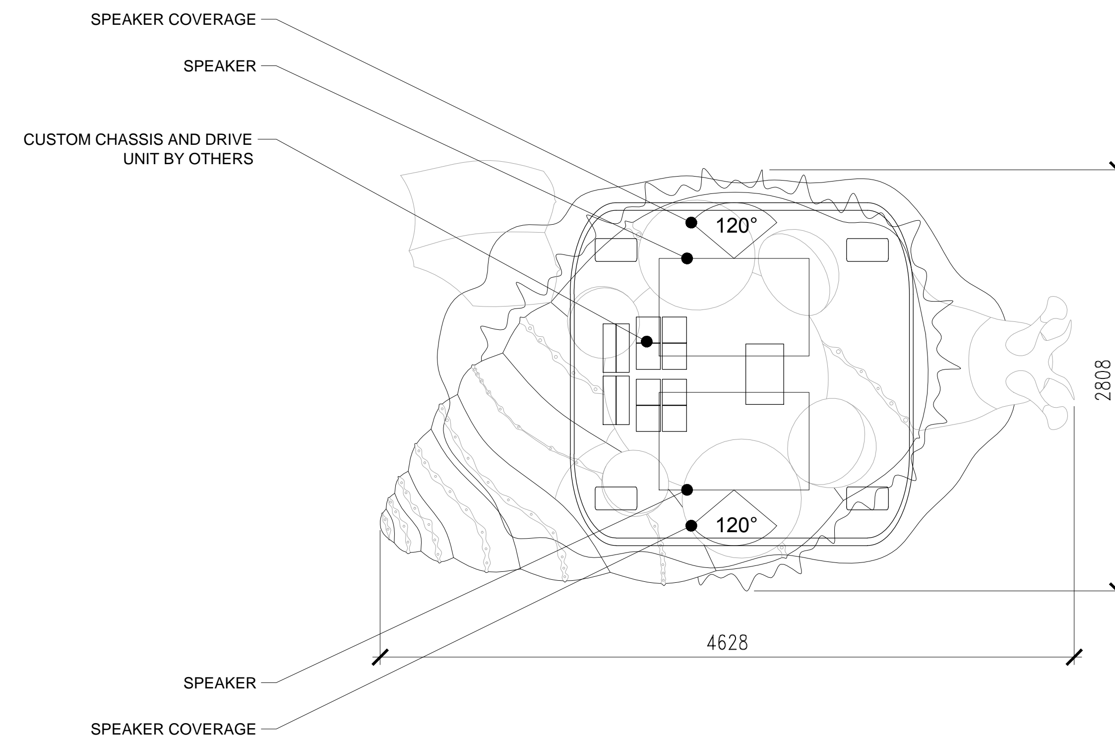
4 CHIMELONG PARADE CRAB CONGA LINE: SEA SNAIL PLAN 1:25
