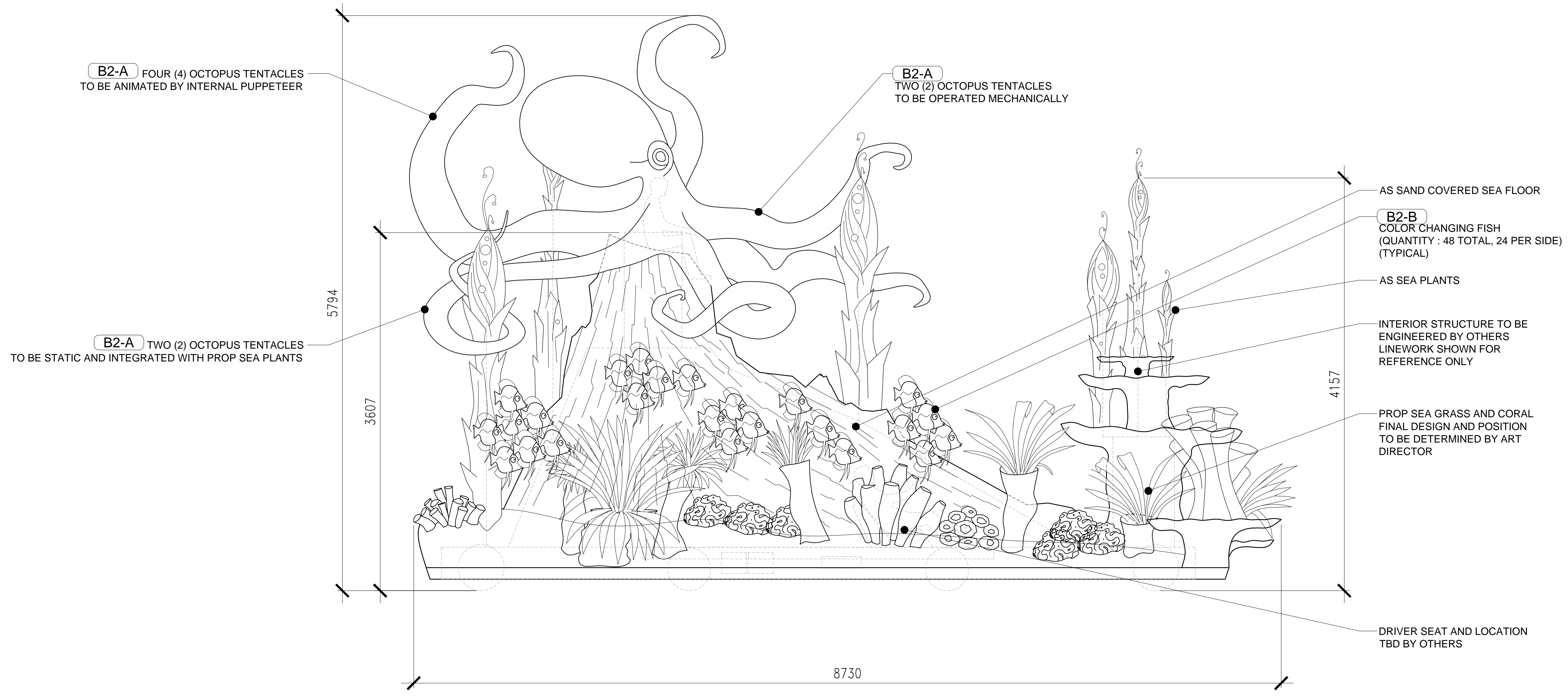
6 CHIMELONG PARADE CORAL REEF: OCTOPUS ELEVATION 1:25
